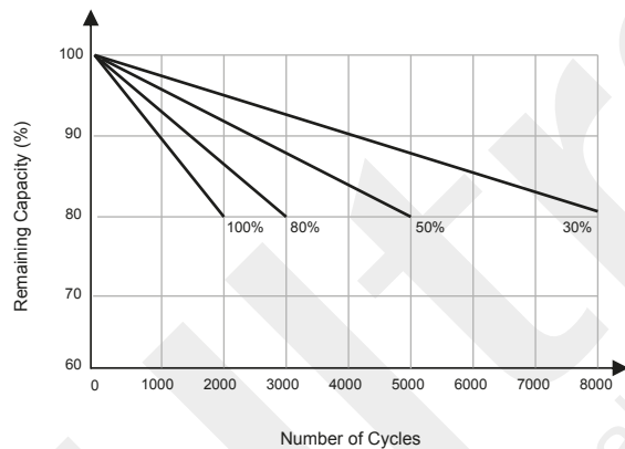
Cycle Life on D.O.D (25°C)
